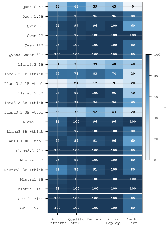
(A) MCQ Accuracy (%)
