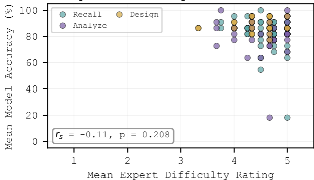
(A) Expert Difficulty vs. Model Accuracy
