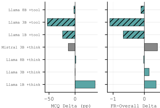
(A) MCQ Accuracy (B) FR-Overall Score
